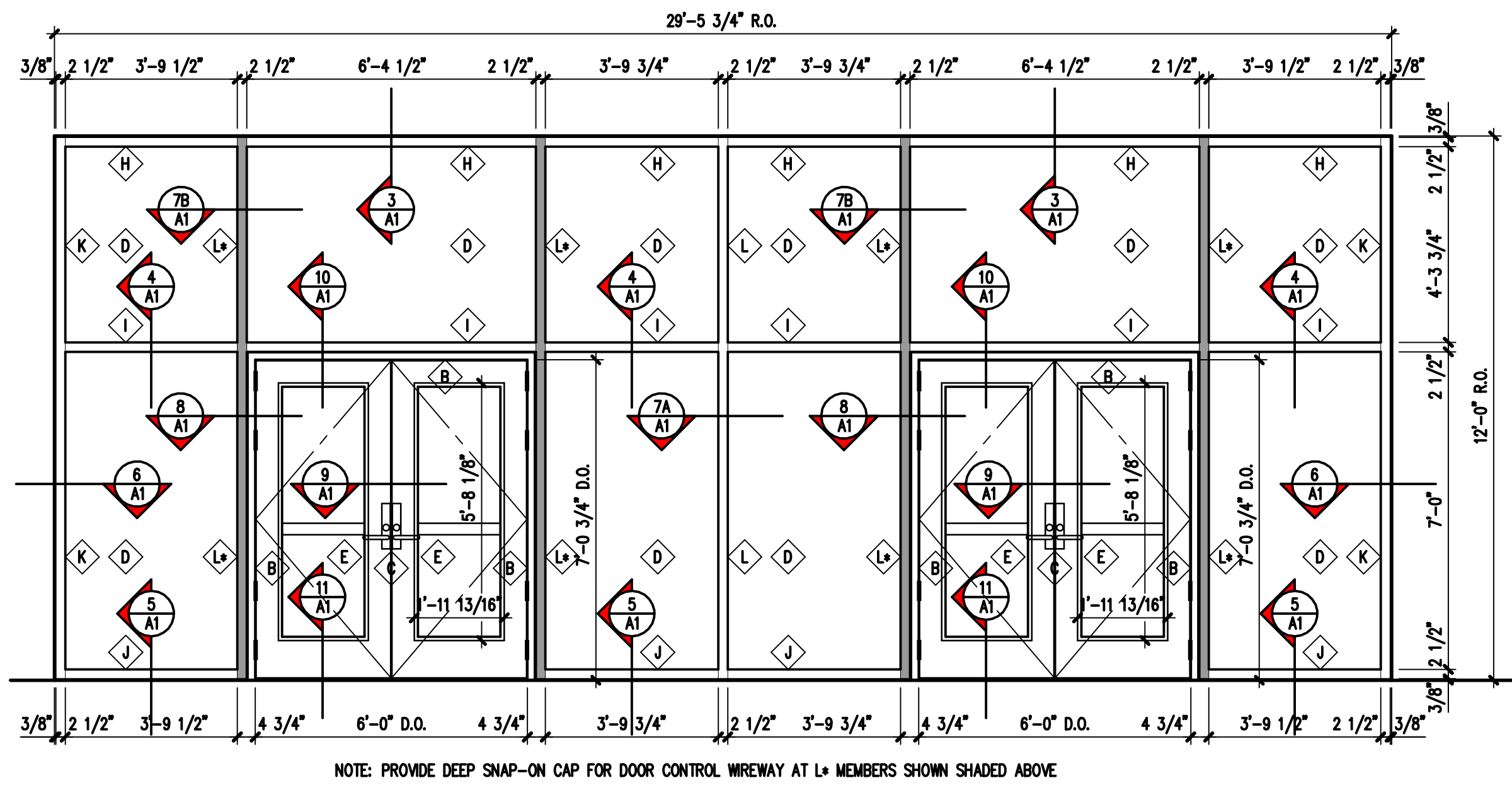
2 FIRE RATED ENTRY SYSTEM ELEVATION 3/8\" = 1'-0"
