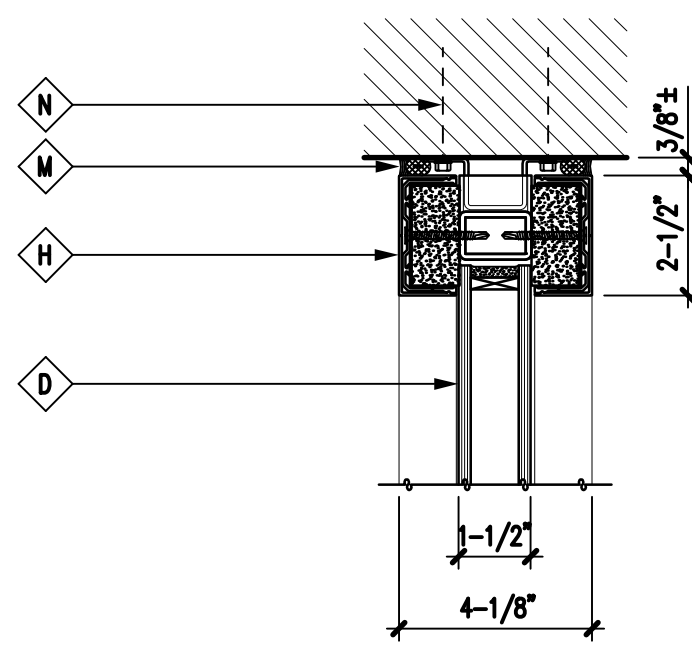
3 TRANSOM HEAD DTL 3\" = 1'-0"
