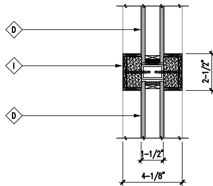
4 HORIZ MULLION DTL 3\" = 1'-0"
