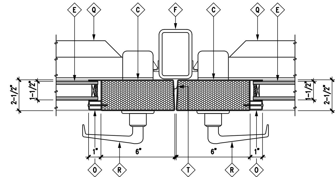
9 DOOR MEETING STILES DTL 3\" = 1'-0"
