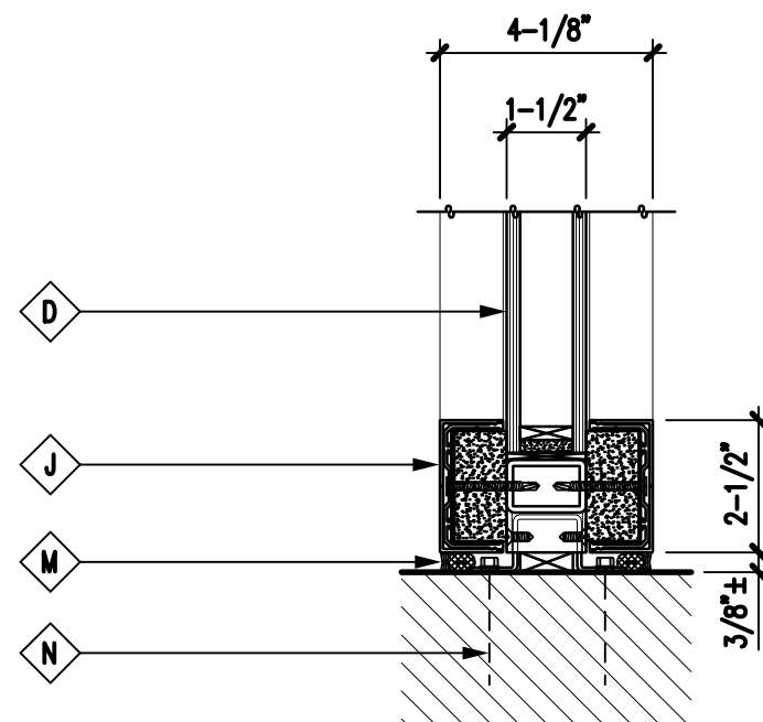
5 SILL DTL 3\" = 1'-0"
