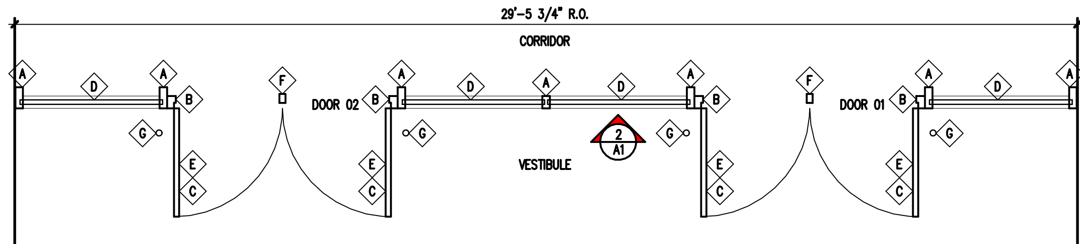
1 FIRE RATED ENTRY SYSTEM PLAN 3/8\" = 1'-0"
