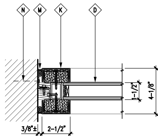
5 SILL DTL 3\" = 1'-0"
