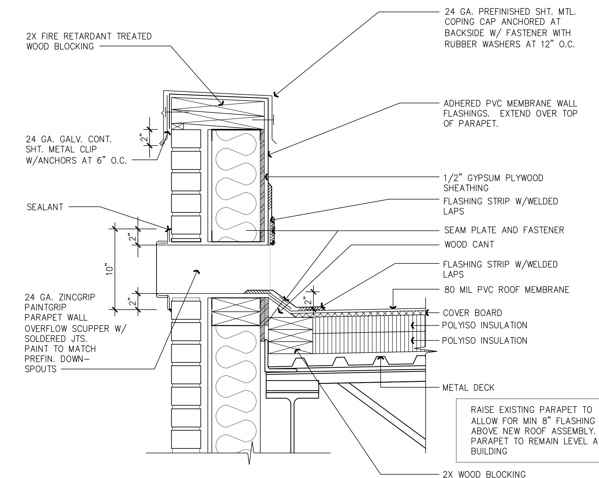
01 THRU-WALL OVERFLOW SCUPPER DETAIL
