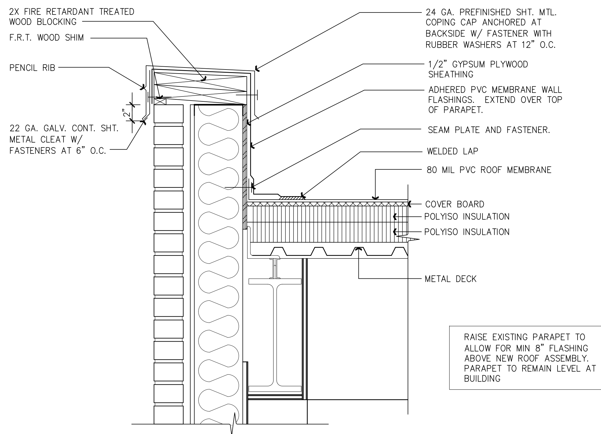
02 PARAPET DETAIL
