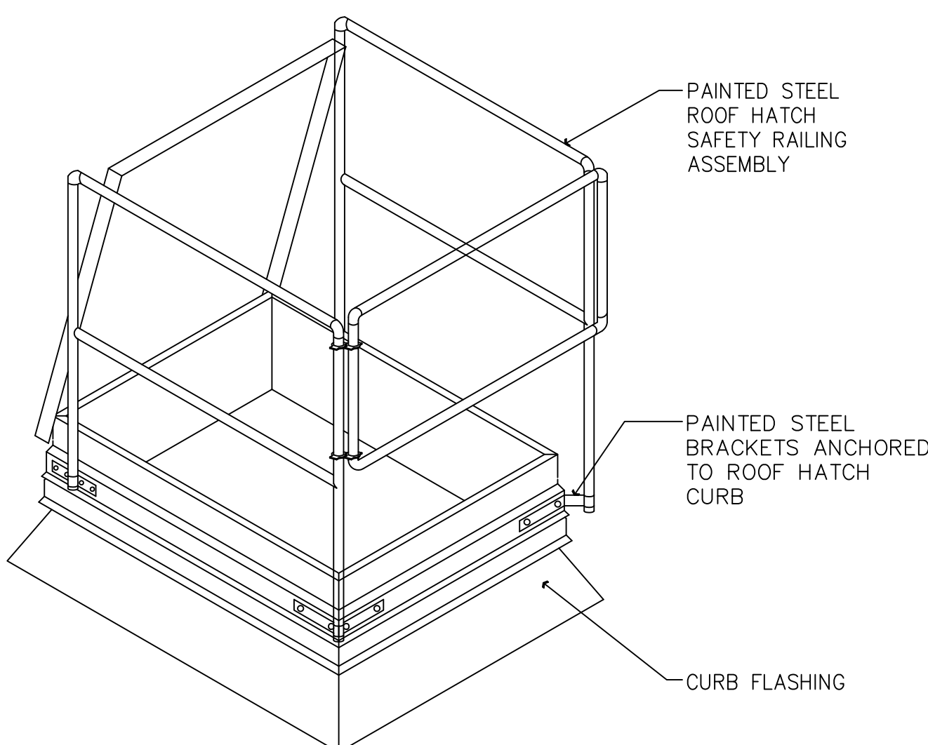
05 ROOF HATCH SAFETY RAILING
