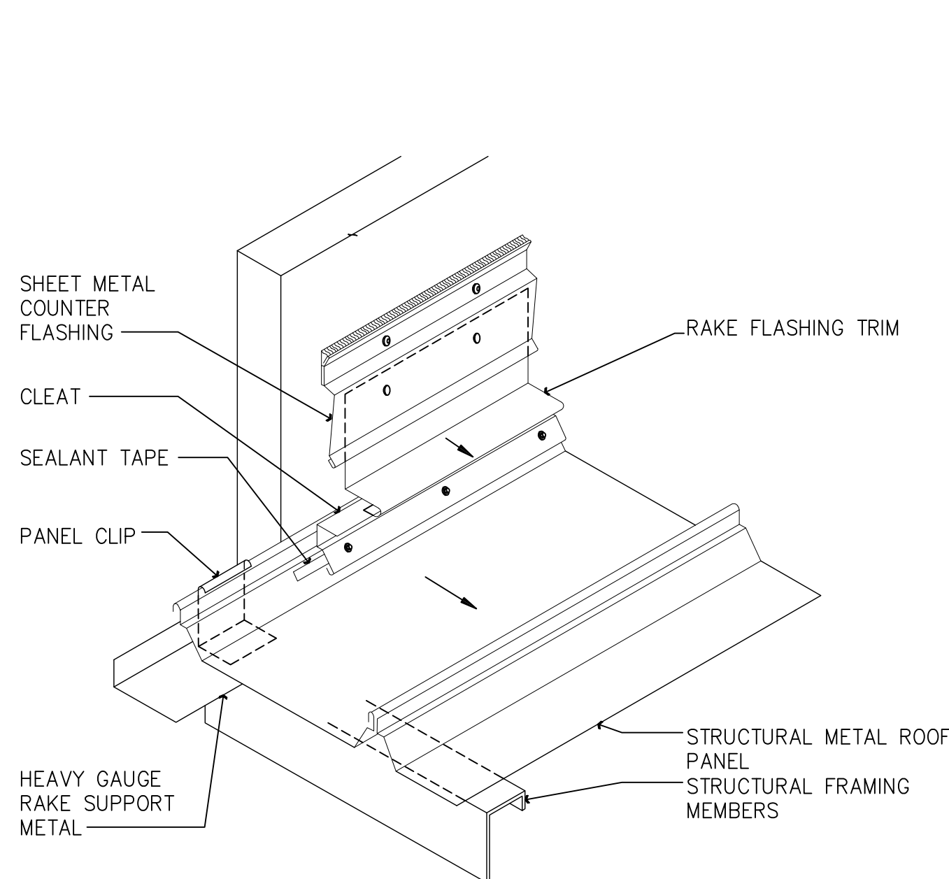
07 SIDEWALL TRANSITION DETAIL
