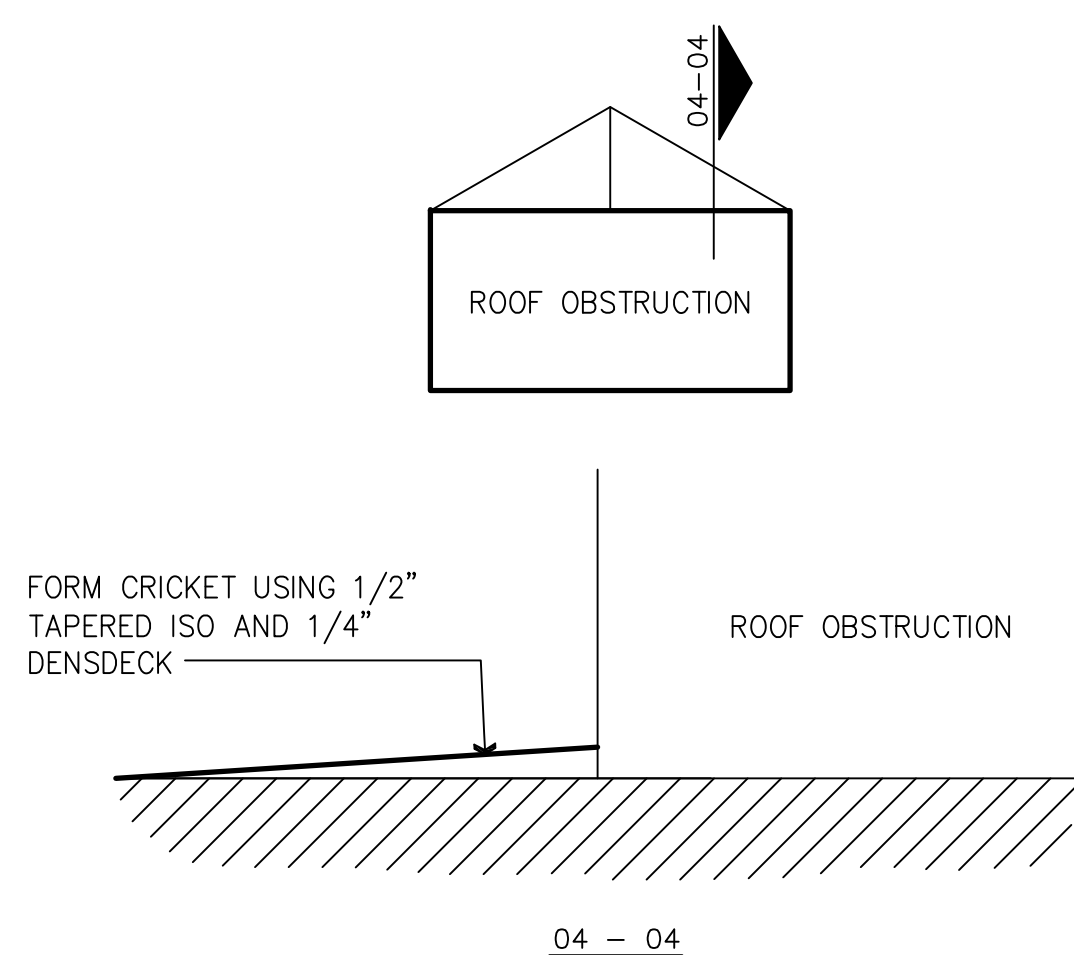
02 CRICKET DETAIL SCALE: 1-1/2" = 1'-0"
