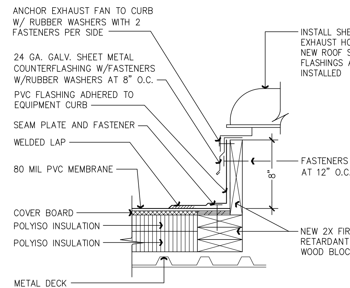
10 EXHAUST FAN DETAIL SCALE: 1-1/2" = 1'-0"
