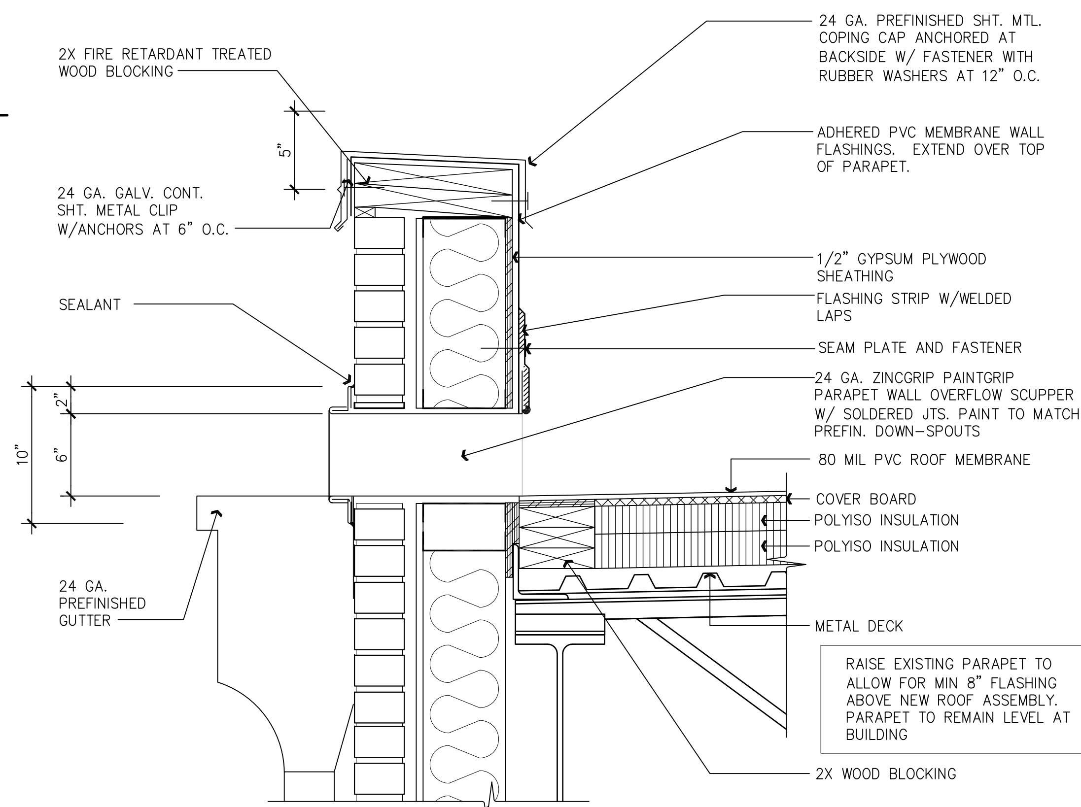
04 THRU-WALL SCUPPER DETAIL
