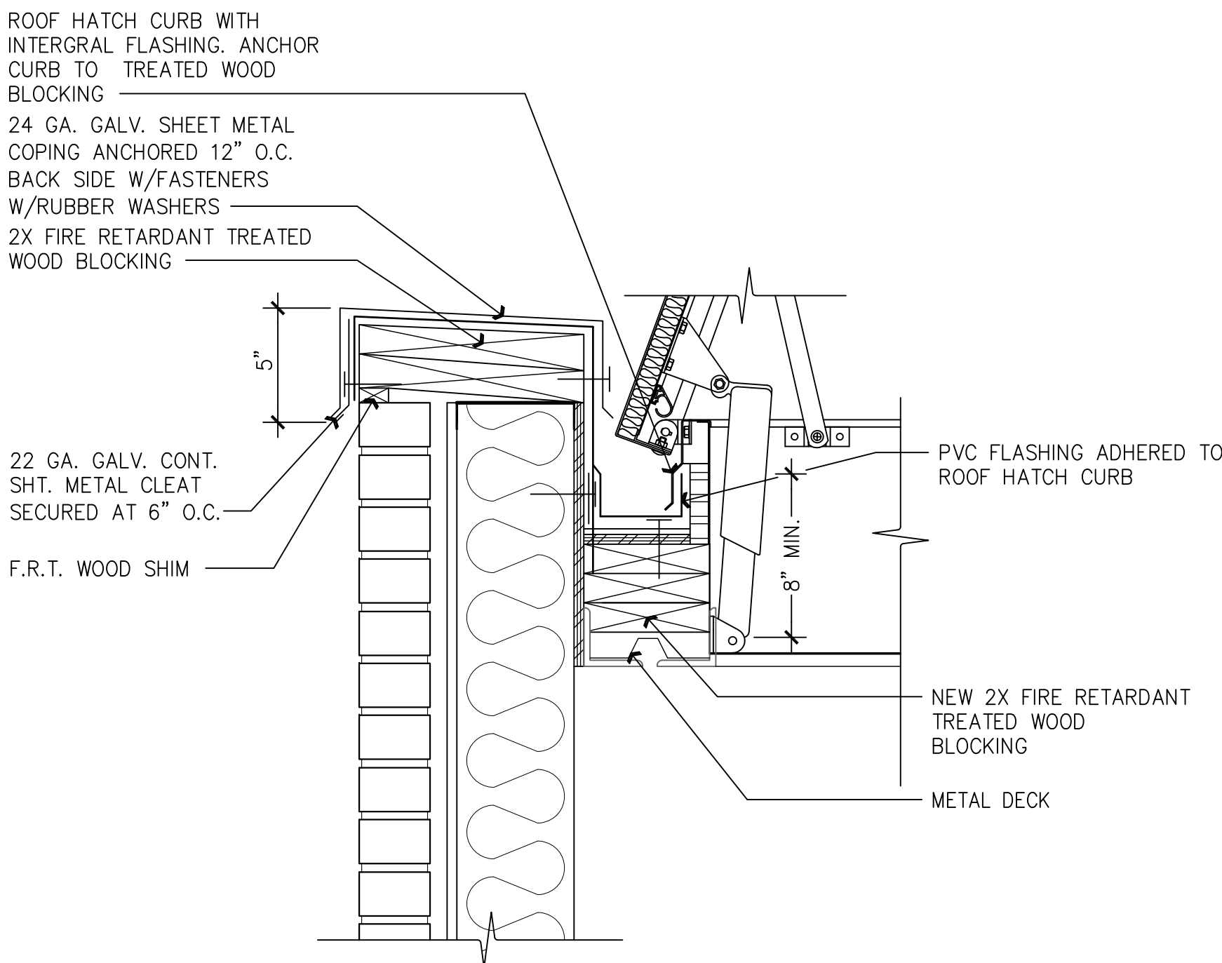
12 ROOF HATCH DETAIL SCALE: 1-1/2" = 1'-0"
