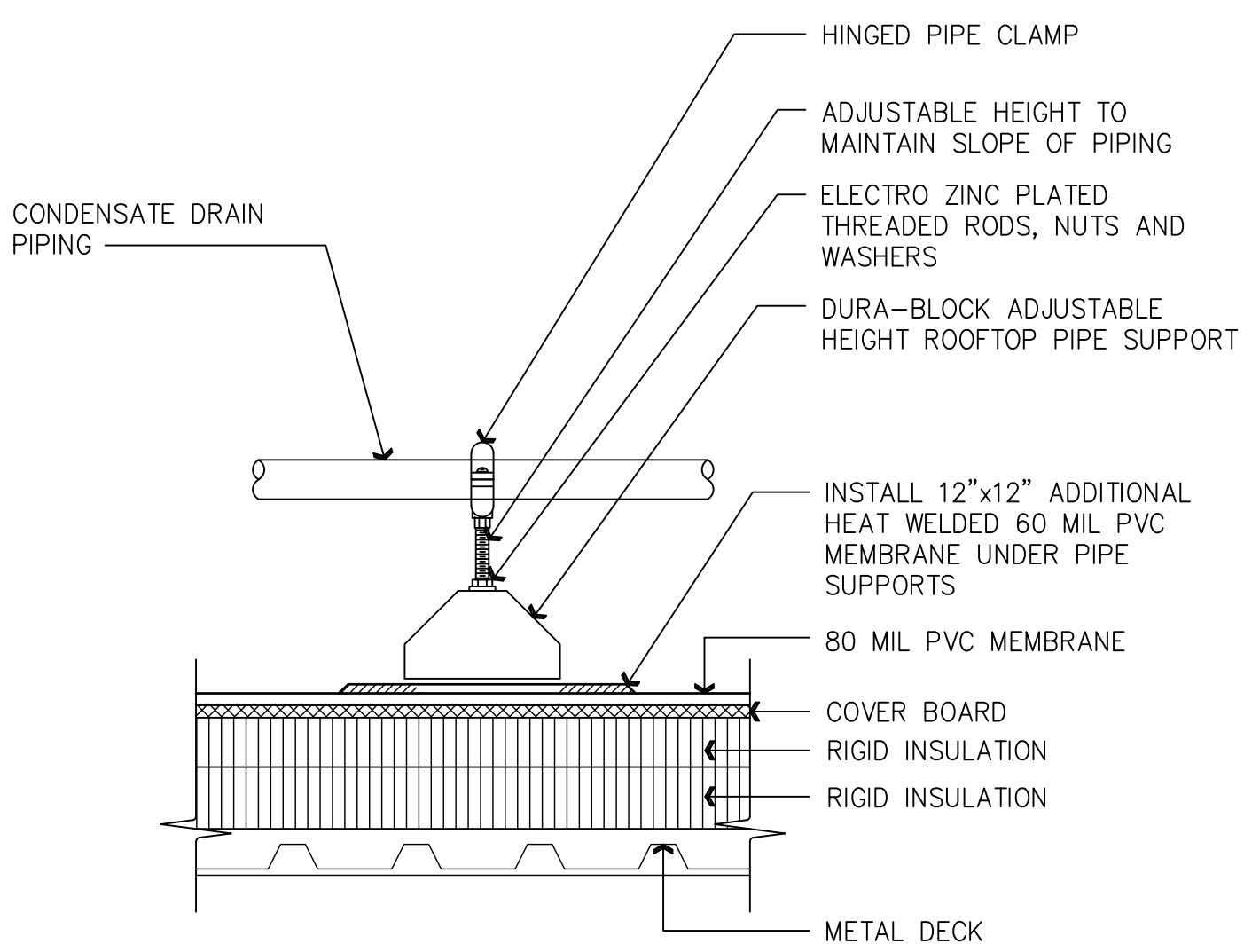
08 PIPE SUPPORT DETAIL SCALE: 1-1/2" = 1'-0"
