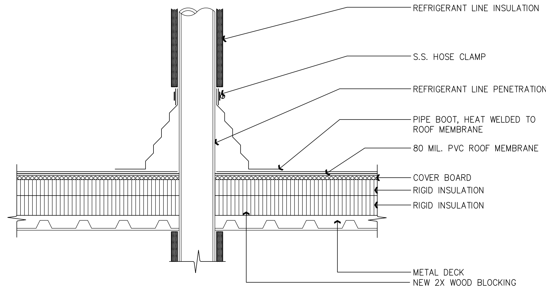
03 PIPE PENETRATION DETAIL SCALE: 1-1/2" = 1'-0"
