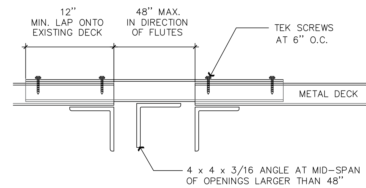
01 ROOF REPAIR DETAIL SCALE: 1-1/2" = 1'-0"
