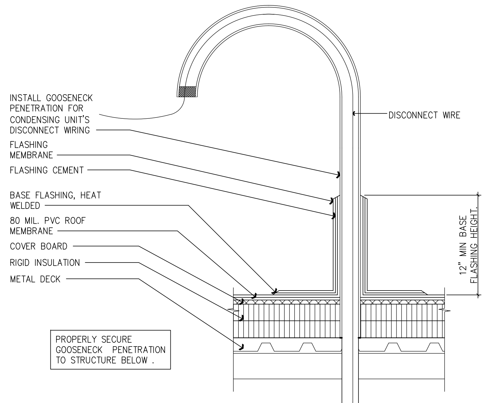
11 GOOSENECK PENETRATION DETAIL SCALE: 1-1/2" = 1'-0"
