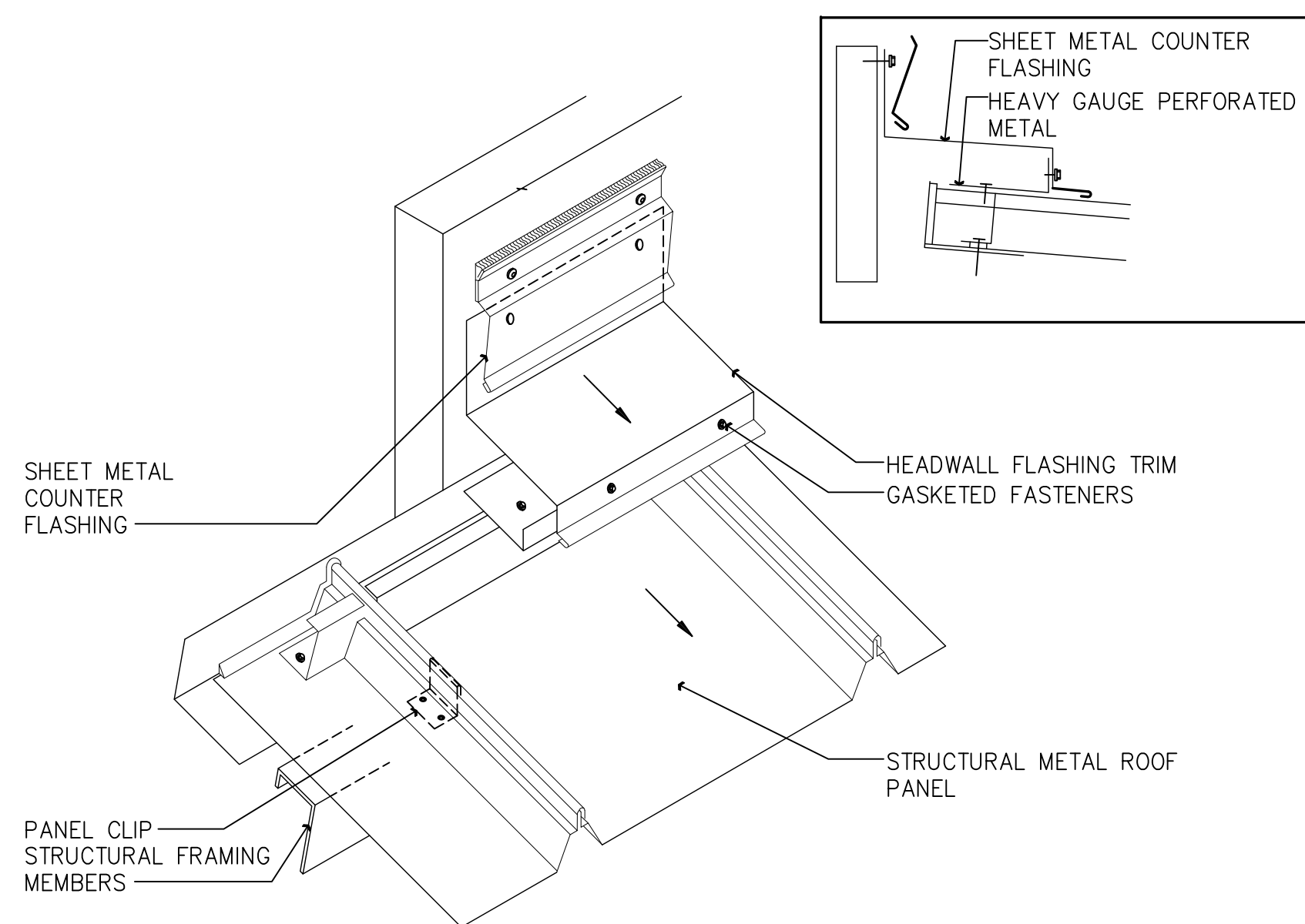
06 HEADWALL TRANSITION DETAIL
