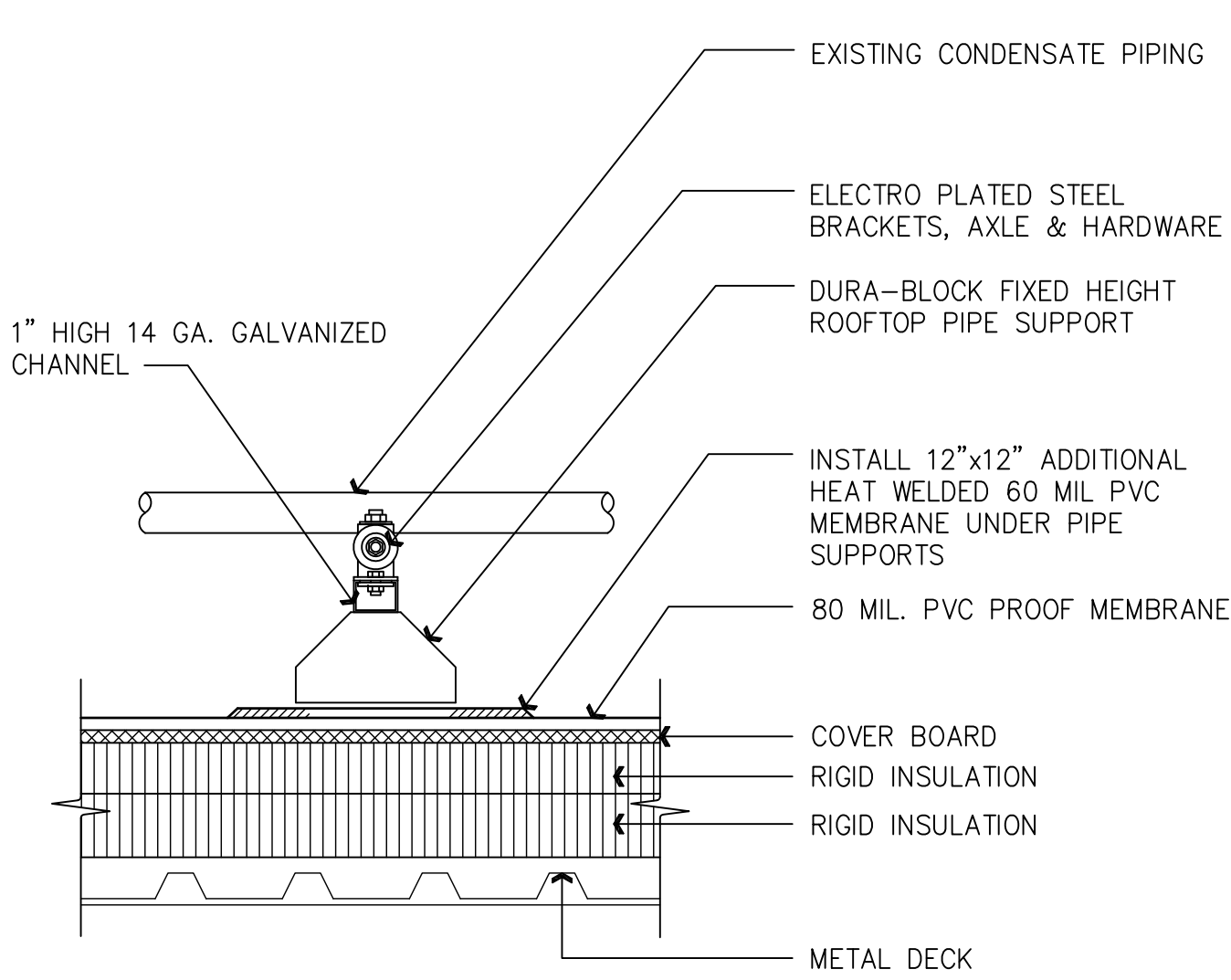
07 PIPE SUPPORT DETAIL SCALE: 1-1/2" = 1'-0"
