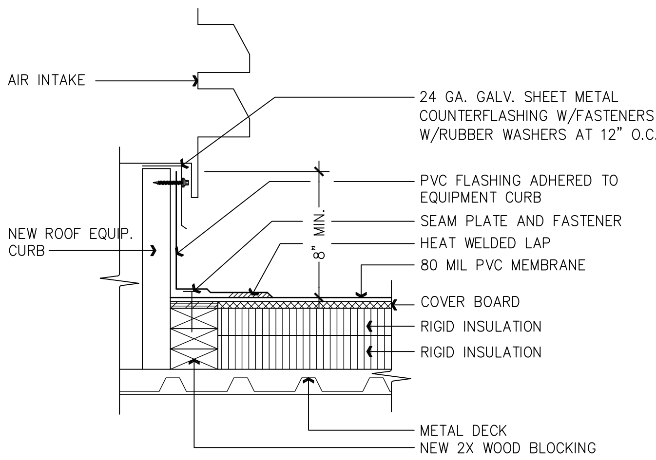
04 INTAKE VENT DETAIL SCALE: 1-1/2" = 1'-0"
