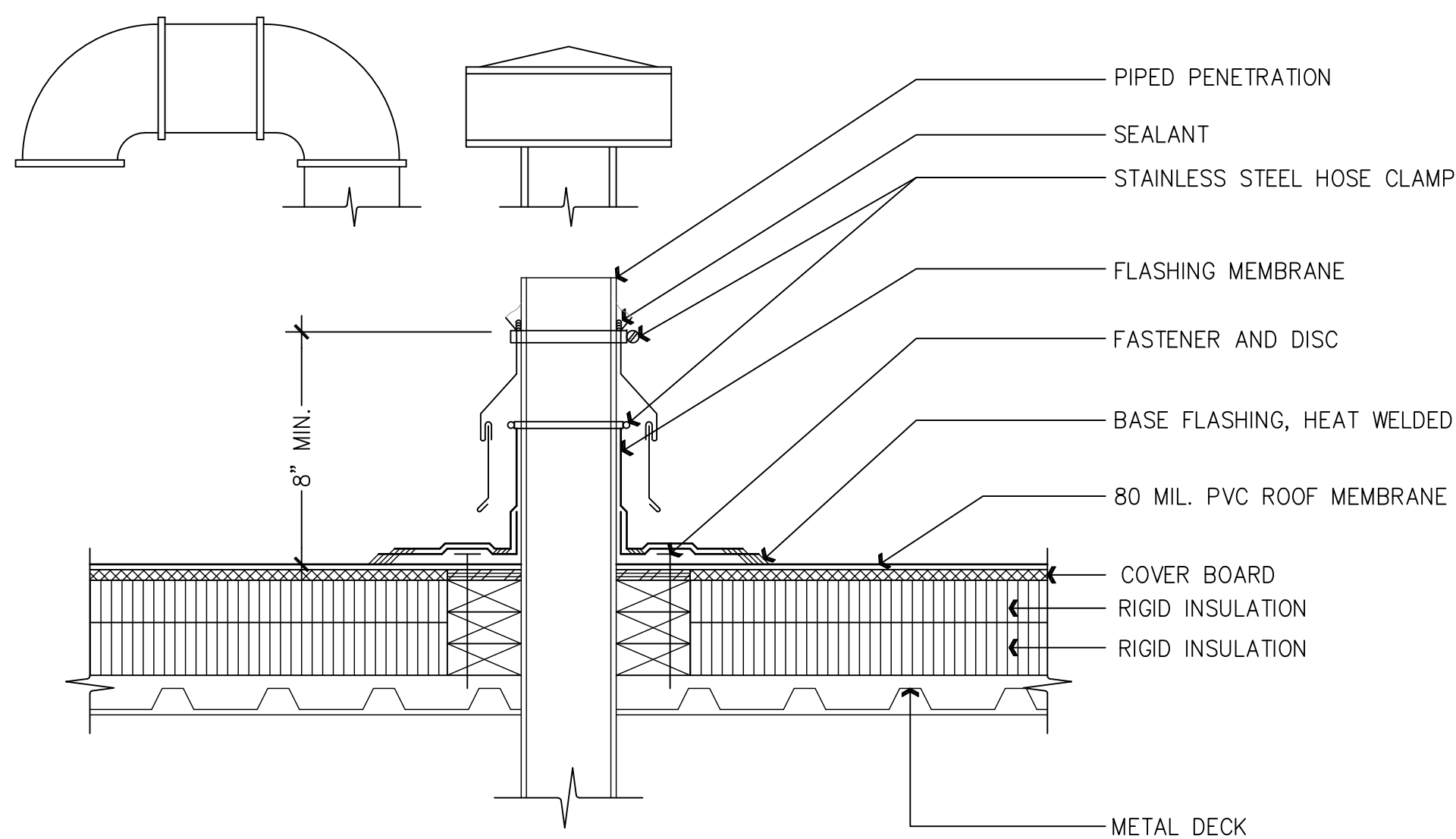
06 PIPE PENETRATION DETAIL SCALE: 1-1/2" = 1'-0"
