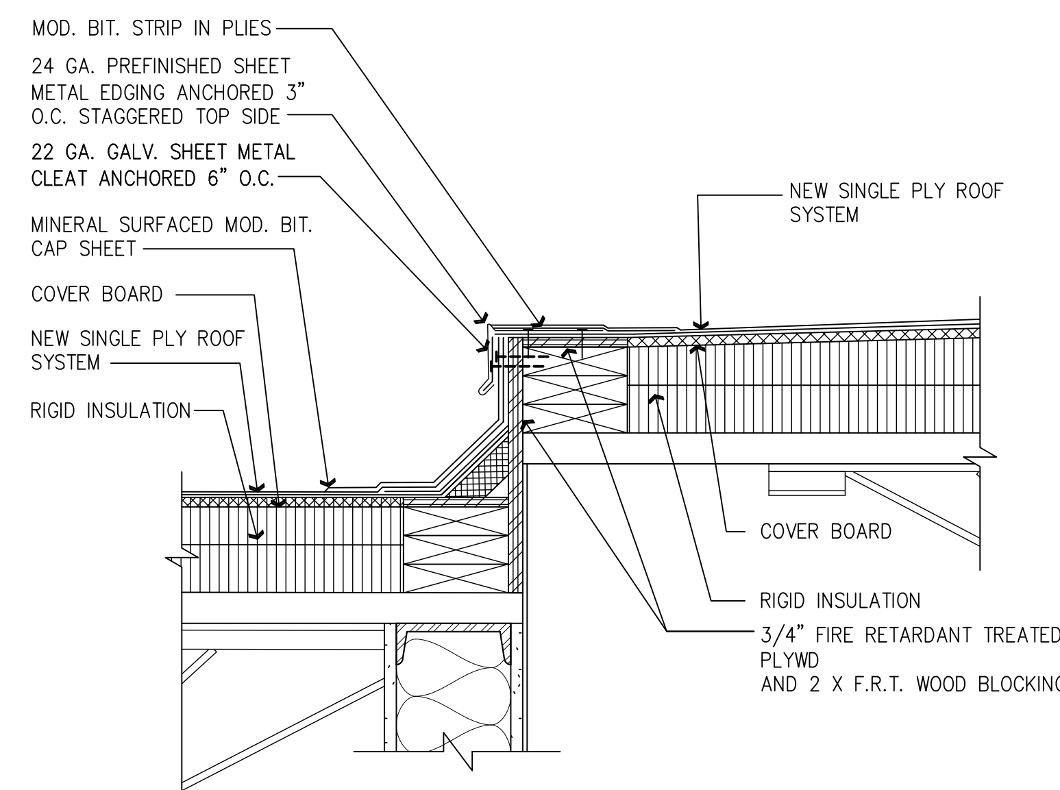
13 DETAIL AT CHANGE IN ELEVATION SCALE: 1-1/2" = 1'-0"
