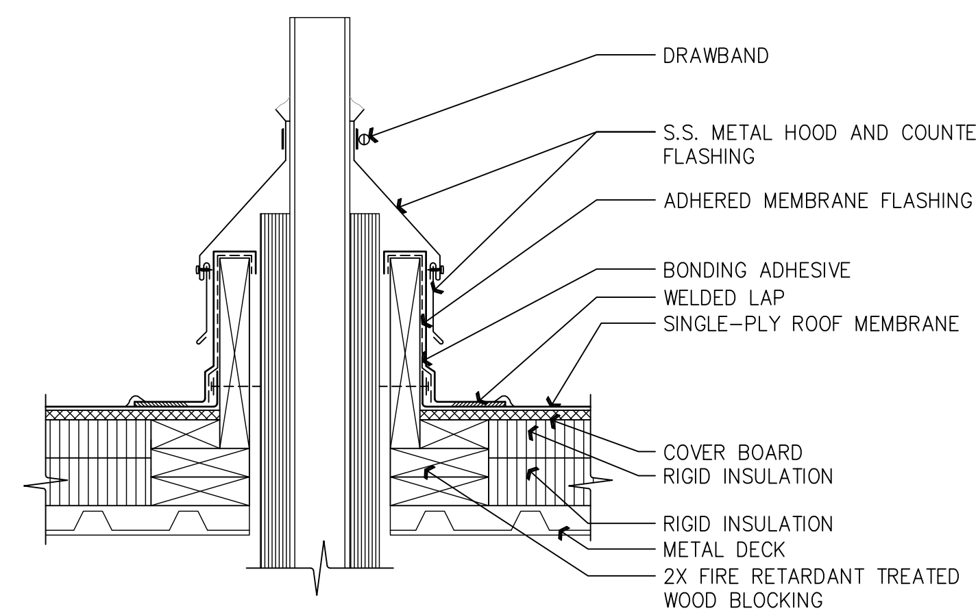
05 HOT STACK PIPE PENETRATION DETAIL SCALE: 1-1/2" = 1'-0"
