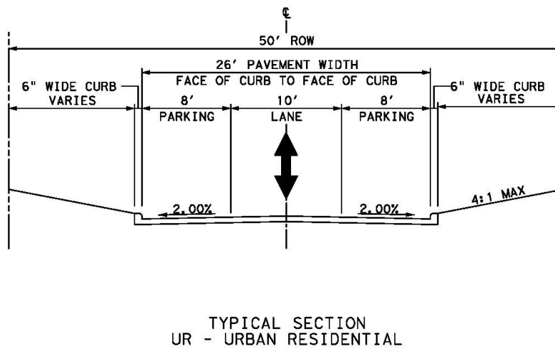
Figure 1.04-2 Typical Geometric Section for Urban Residential Roadways - UR
