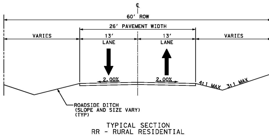
Figure 1.04-1 Typical Geometric Section for Rural Residential Roadways - RR
