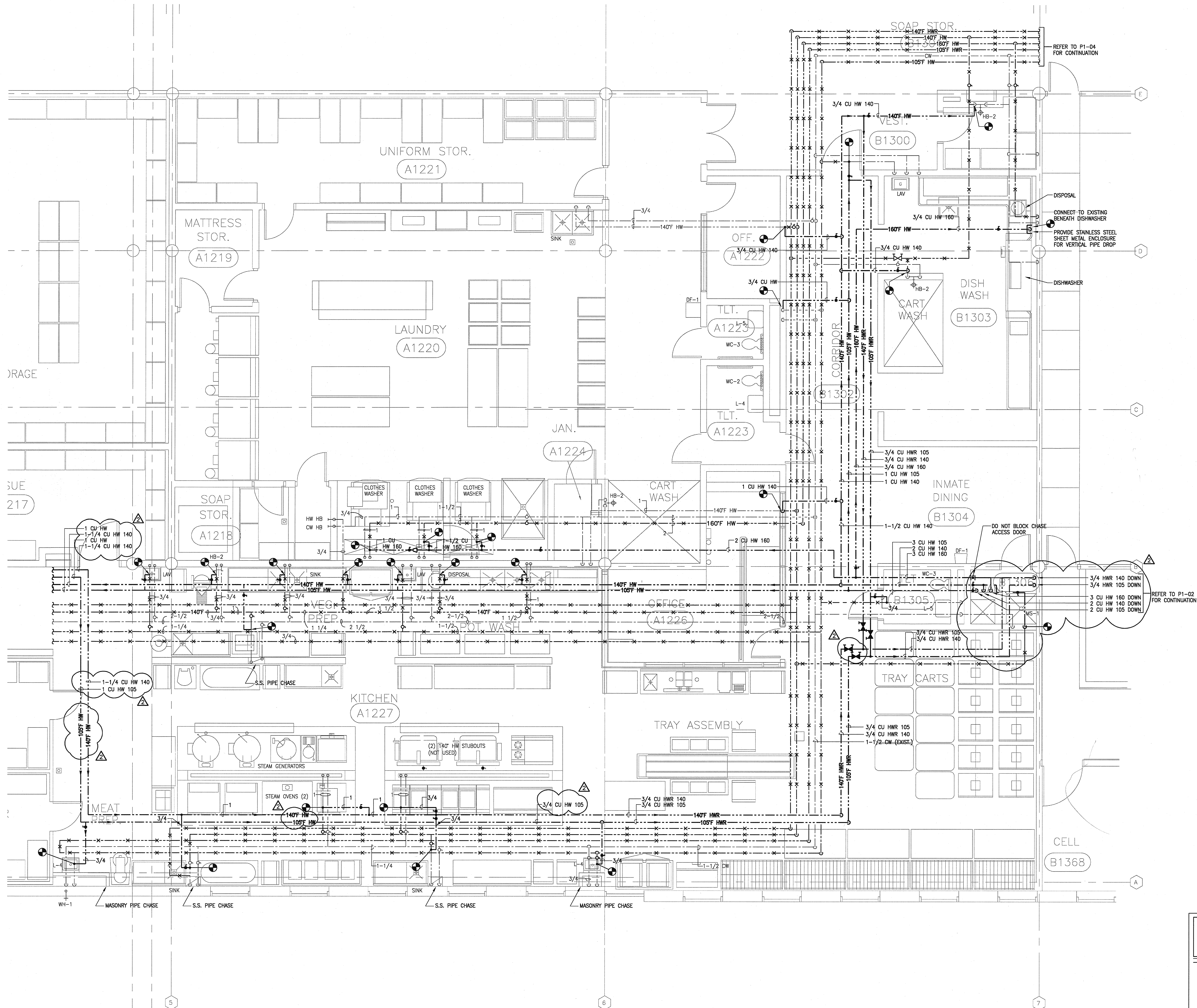
01 ENLARGED KITCHEN & LAUNDRY PLUMBING PLAN SCALE: 1/4" = 1'-0"
