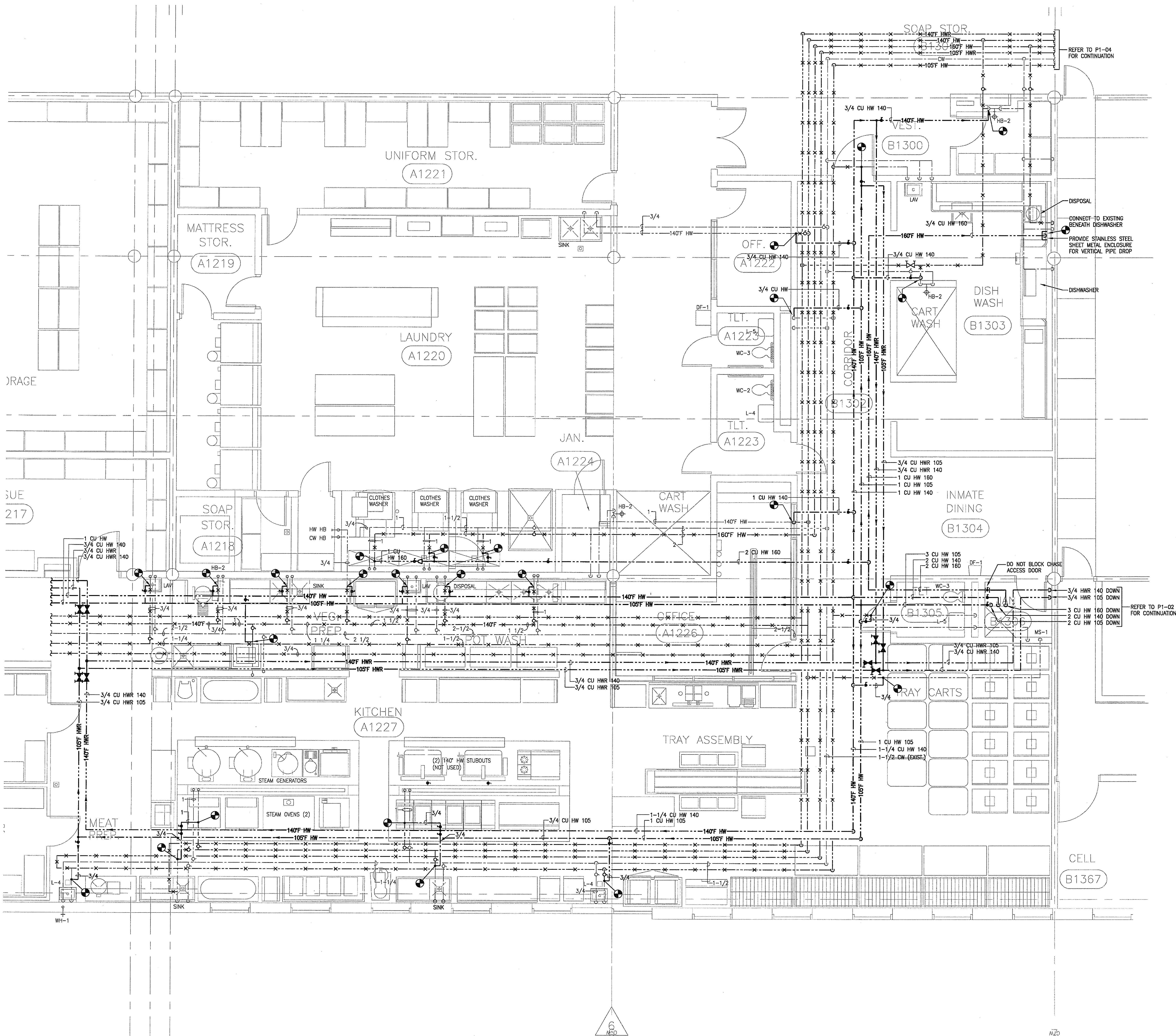
01 ENLARGED KITCHEN & LAUNDRY PLUMBING PLAN SCALE: 1/4" = 1'-0"
