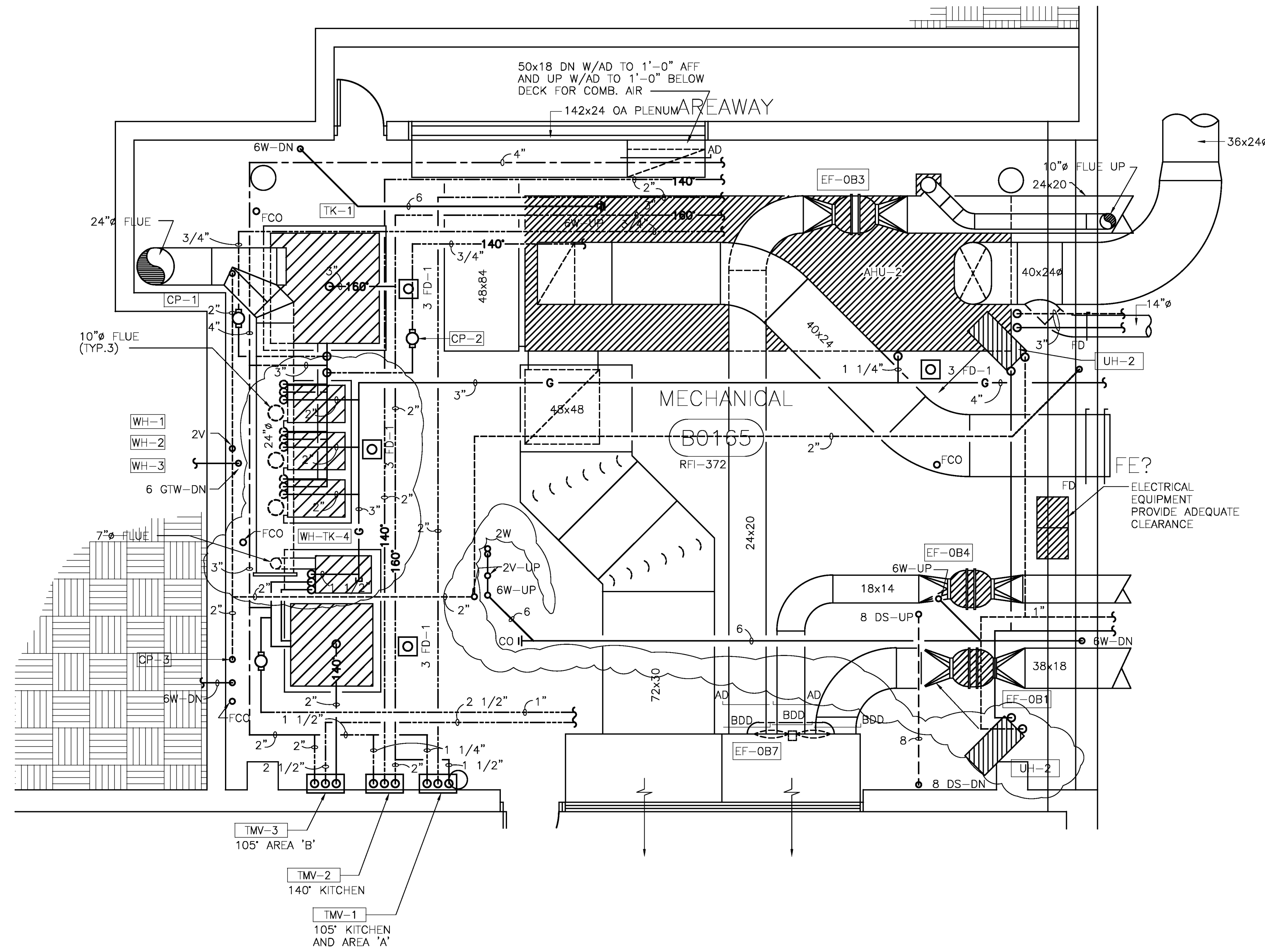
LOWER LEVEL MECHANICAL ROOM
