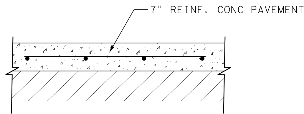
EXISTING CONCRETE PAVEMENT SECTION
