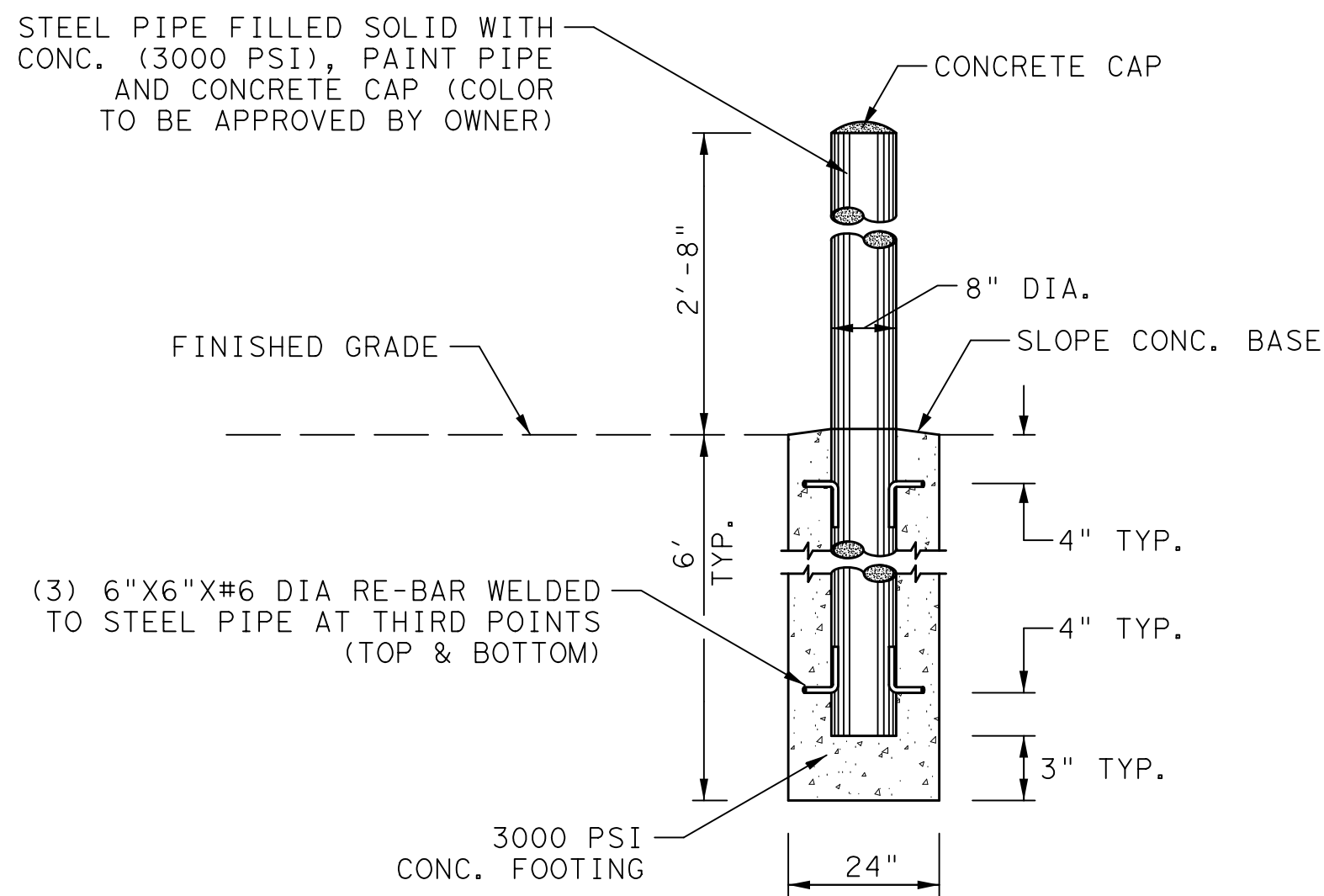
PIPE BOLLARD DETAIL
