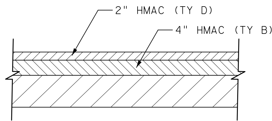
EXISTING ASPHALT PAVEMENT SECTION
