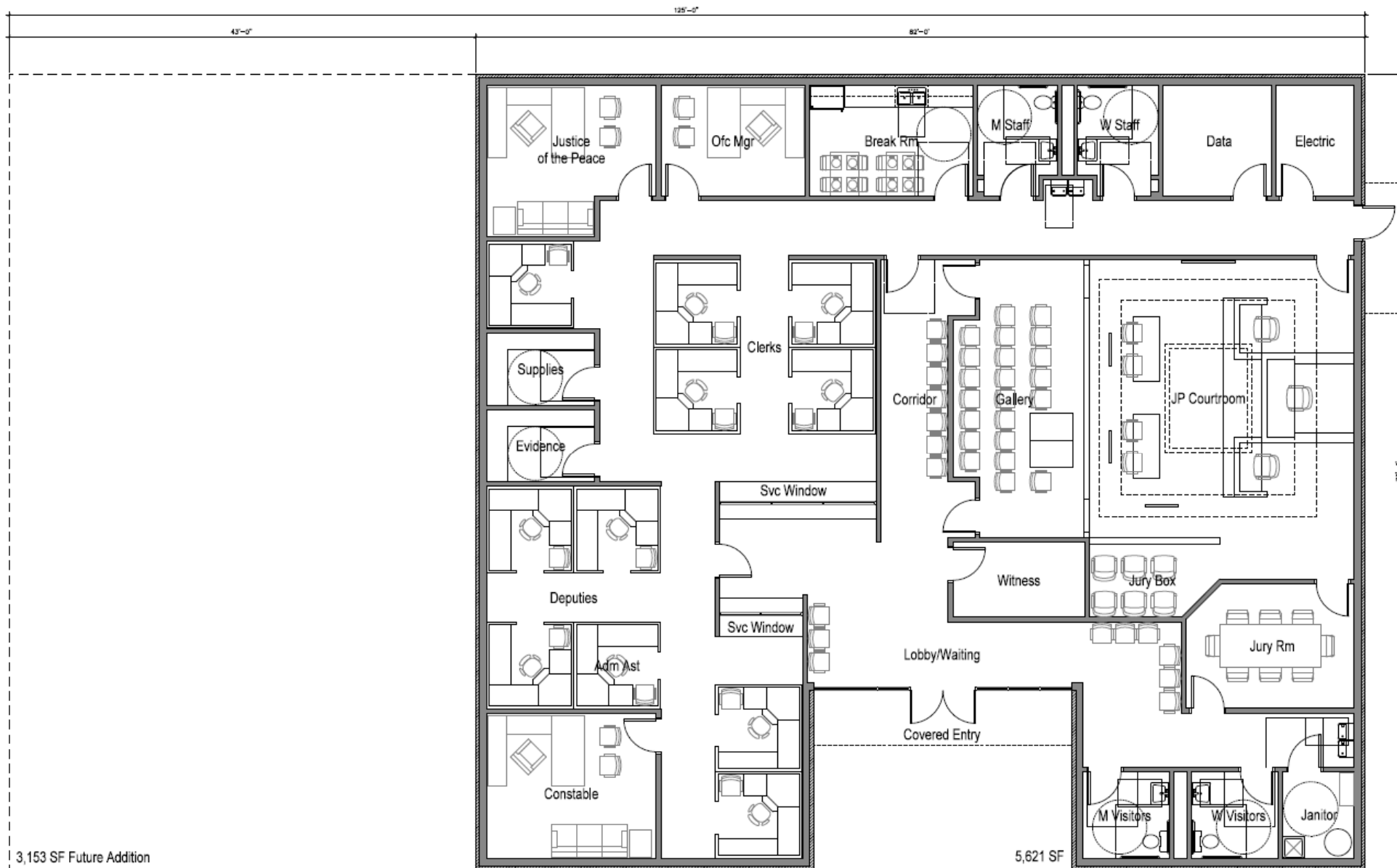
FLOOR PLAN A - REV 29JAN19
